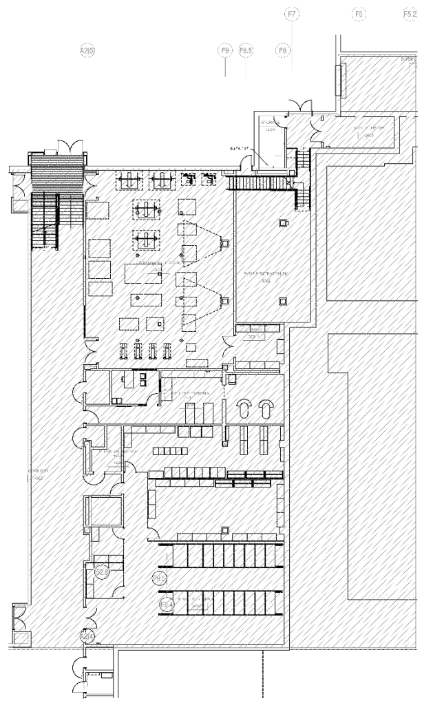
LEVEL 0 ELECTRICAL PLAN - NEW WORK SCALE: 1/8" = 1'-0"
